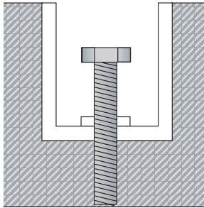
Adjusting bolt
