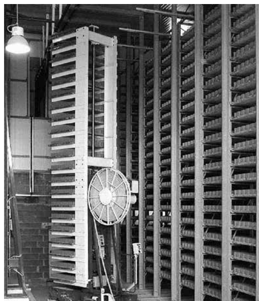
Safe in- and output by means of the finger car and the HS-guiding-rails.
