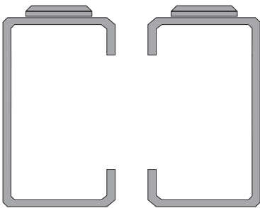
Left and right support profile (steel support)
